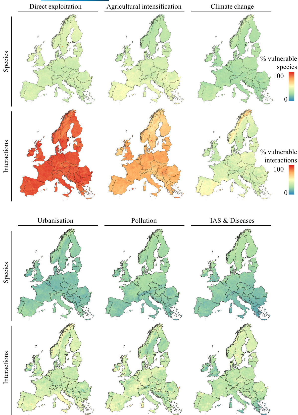
FIGURE 4 Maps of the vulnerability of species and interactions across Europe to the six major threats. Top row: Percentage of species in the grid cell that are vulnerable to each threat. Bottom row: percentage of interactions in the local food web that the vulnerable species are associated with. The color gradient used is the same for all maps. Map lines delineate study areas and do not necessarily depict accepted national boundaries. IAS, invasive alien species.
